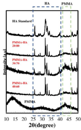
Figure 1. XRD pattern of pure PMMA, HA, and PMMA-HA sample for 20:80; 30:70 and 40:60 ratio.
