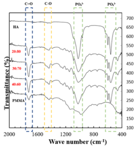
Figure 2. FTIR pattern of pure PMMA, HA, and PMMA-HA sample for 20:80; 30:70 and 40:60 ratio.
