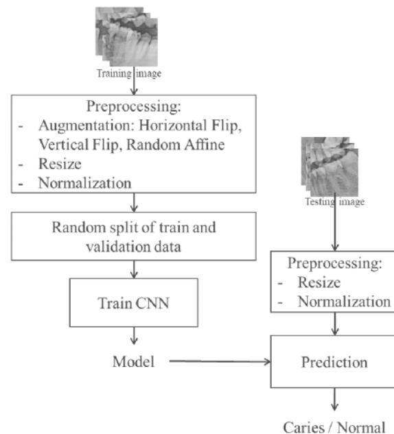
Fig. 1 Design System
