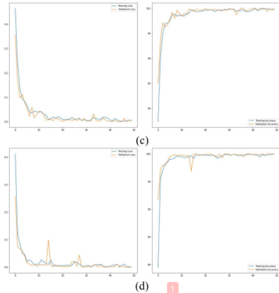
Fig. 8 Training loss and validation result (a) 3-layer CNN; (b) 3-layer CNN with batch normalization; (c) ResNet18; (d) ResNeXt50 32x4d
