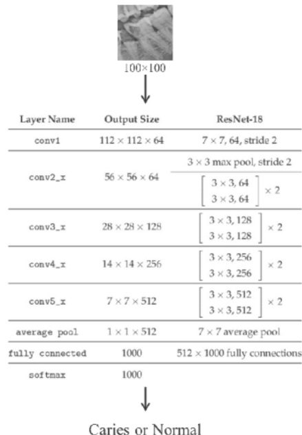
Fig. 6 Resnet18 architecture
