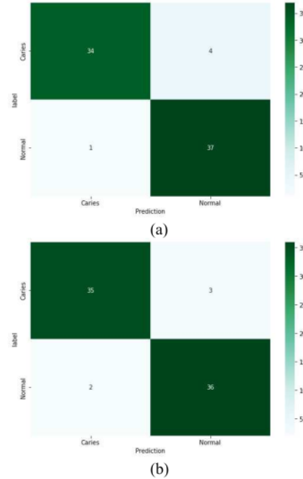
Fig. 9 Confusion matrix (a) ResNet18; (b) ResNeXt50 32x4d
