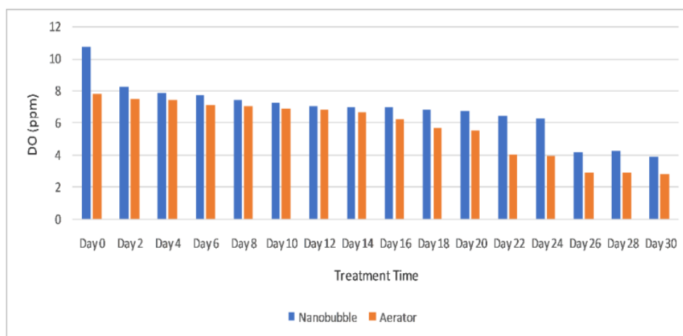
Figure 1. Graph of dissolved oxygen content.
