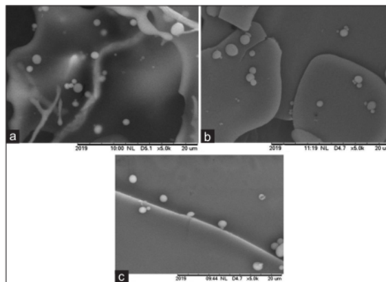
Figure 3: Morphological of ciprofloxacin HCl-carrageenan microspheres Formula 1 (a), Formula 2 (b), and Formula 3 (c) with a magnification of ×5000
