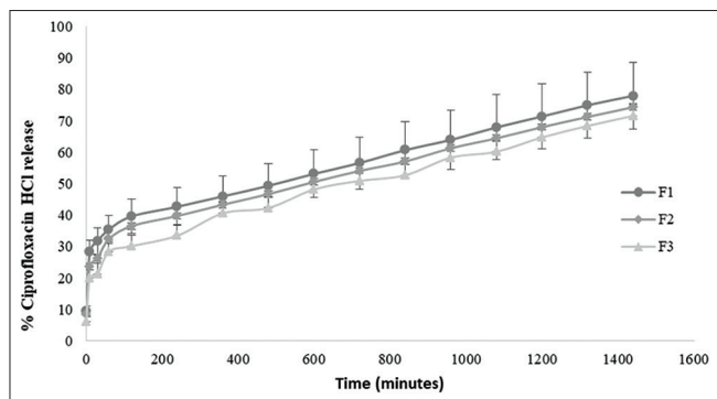
Figure 6: Release of ciprofloxacin HCl from microspheres
