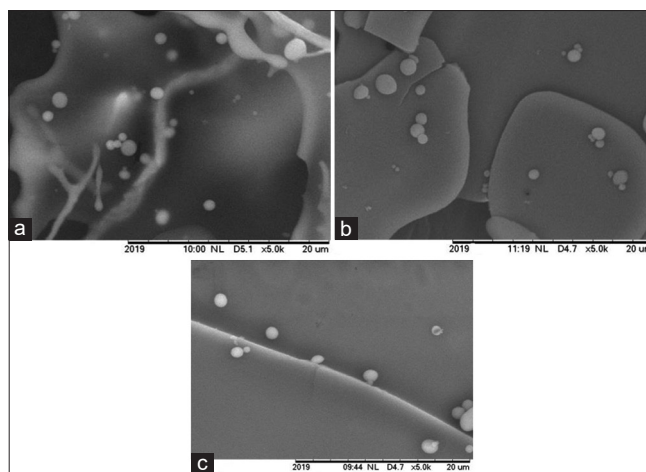
Figure 3: Morphological of ciprofloxacin HCl-carrageenan microspheres Formula 1 (a), Formula 2 (b), and Formula 3 (c) with a magnification of \times 5000
