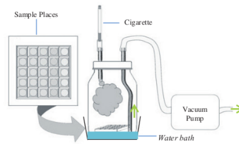
Figure 1. The smoking machine used in this research. 14
