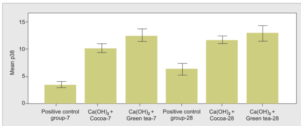
Fig. 6: Graph of mean value of p38 calculation on day 7th and 28th
