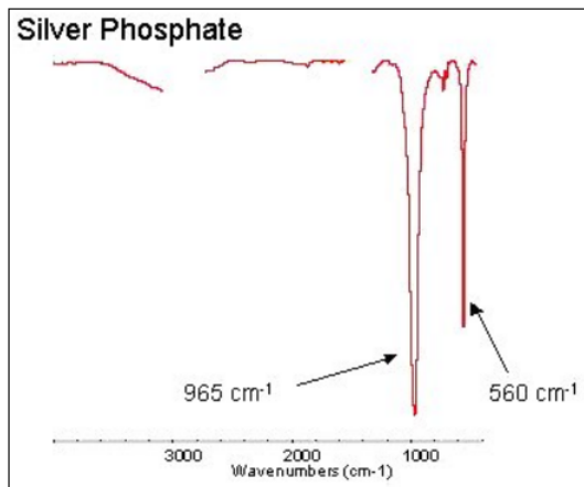
Figure 8. Silver phosphate
