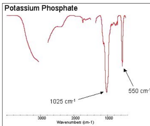
Figure 7. Potassium phosphate
