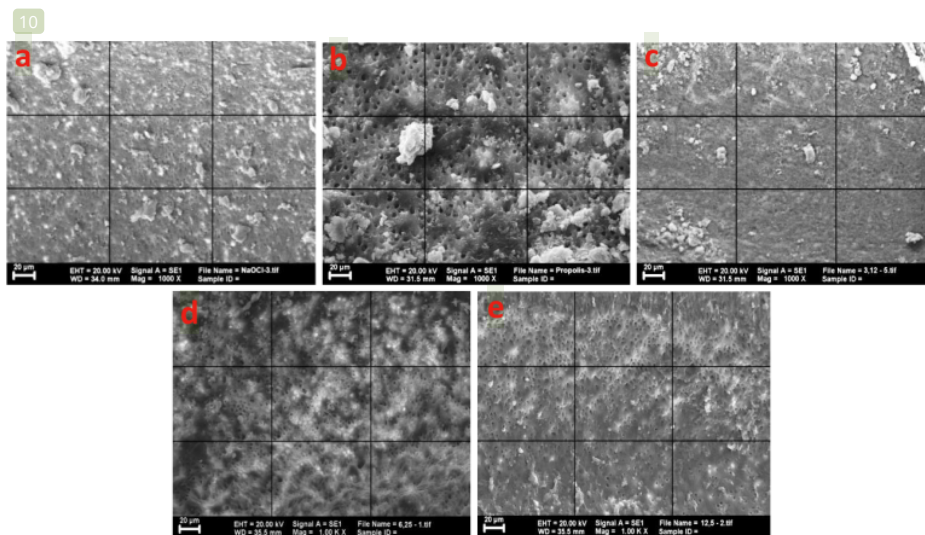
Figure 1. (a) SEM image for control group 2.5% NaOCl; (b) SEM image for 8% propolis; (c) SEM image for 3.12% cocoa; (d) SEM image for 6.25% cocoa; (e) SEM image for 12.50% cocoa.
