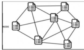
Figure 1. Blockchain System
