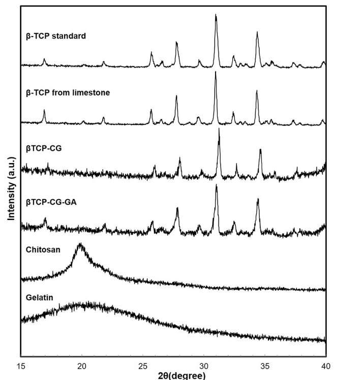
Fig. 2. The XRD patterns of \beta TCP standard, \beta TCP from limestone, \beta TCP-CG scaffold, \beta TCP-CG-GA scaffold, chitosan, and gelatin reference.
