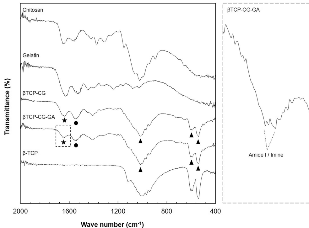
Fig. 3. The FT-IR spectra of chitosan and gelatin reference, \beta TCP-CG, \beta TCP-CG-GA scaffolds, and \beta TCP reference. (▲: phosphate; ★: amide I; ●: amide II).
