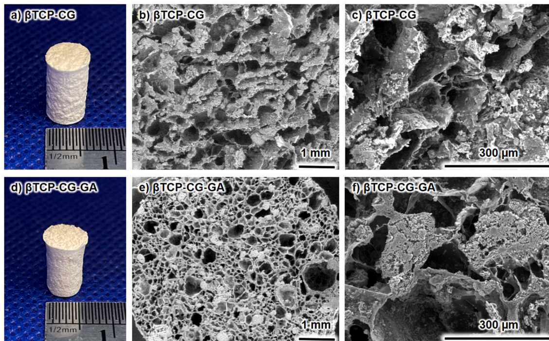
Fig. 1. The photographs of (a) \beta TCP-CG and (d) \beta TCP-CG-GA scaffolds. SEM images of (b, c) \beta TCP-CG and (e, f) \beta TCP-CG-GA scaffolds in low and high magnification.
