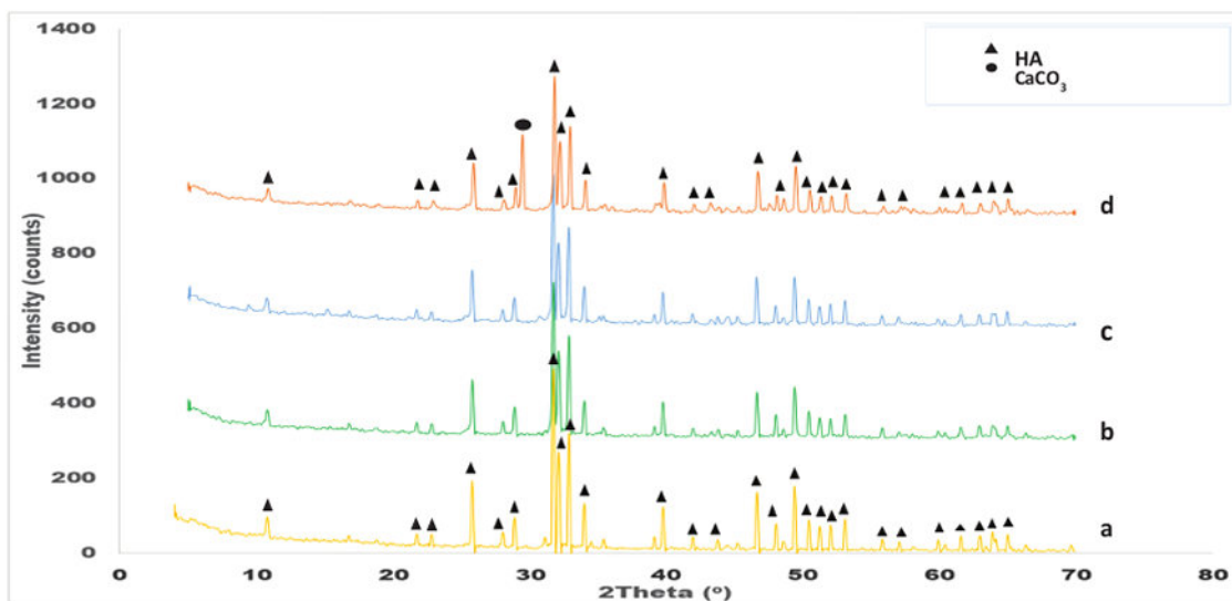
FIGURE 1. XRD pattern of all milled and unmilled materials: (a) HA unmilled, (b) HA milled, (c) HM 48, and (d) HC 48
