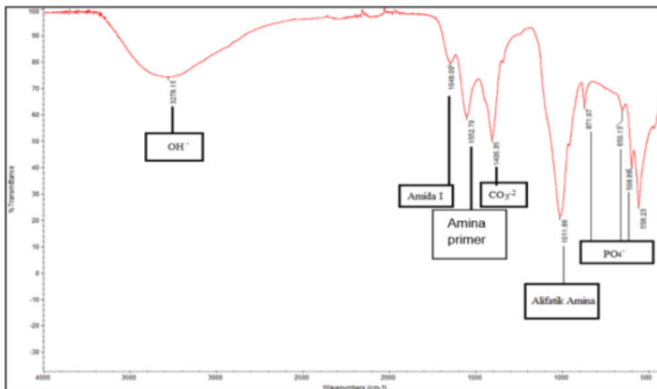
Fig. 4 The results of FTIR test for CA:Ch-GEL scaffold with ratio 80:20
