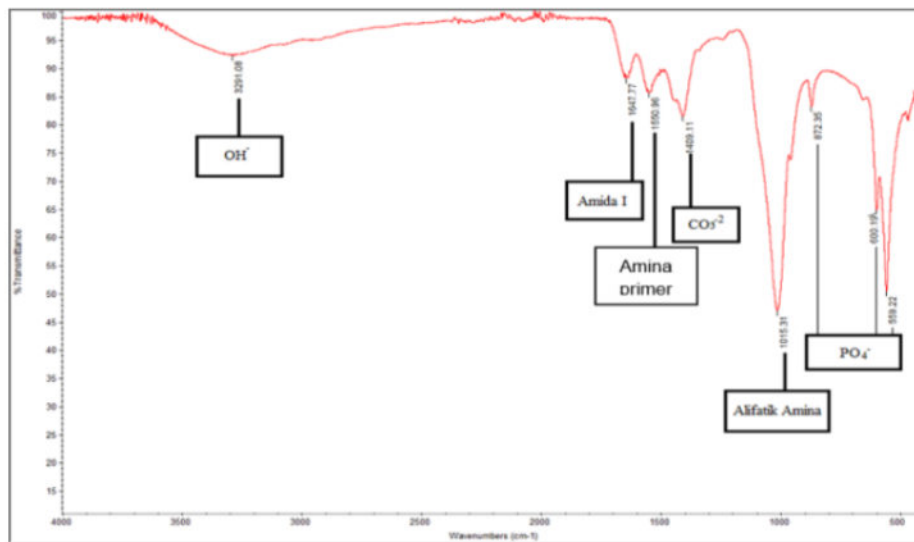
Fig. 3 The results of FTIR test for CA:Ch-GEL scaffold with ratio 70:30
