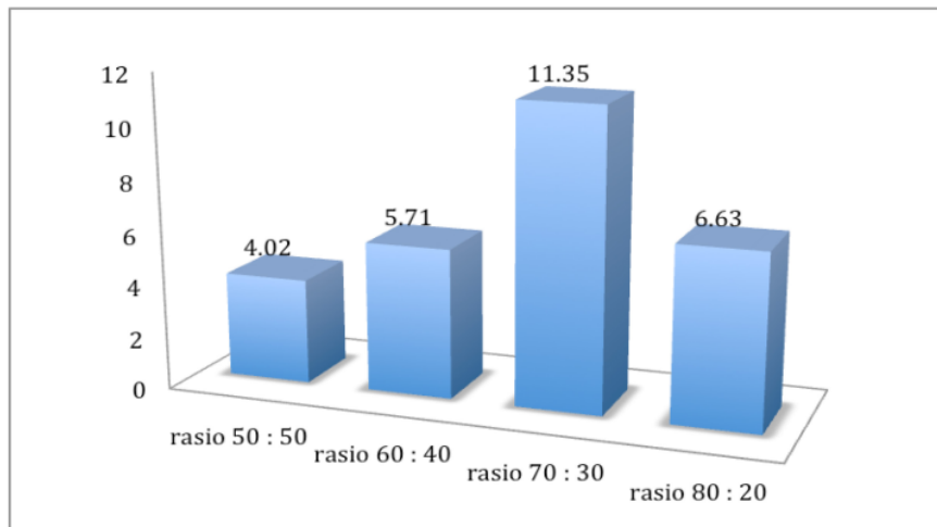
Fig. 5 Compressive strength value of scaffold CA:Ch-GEL
