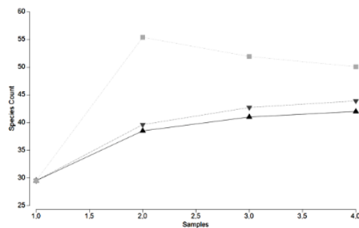
Figure 2. The curves from observed species values
