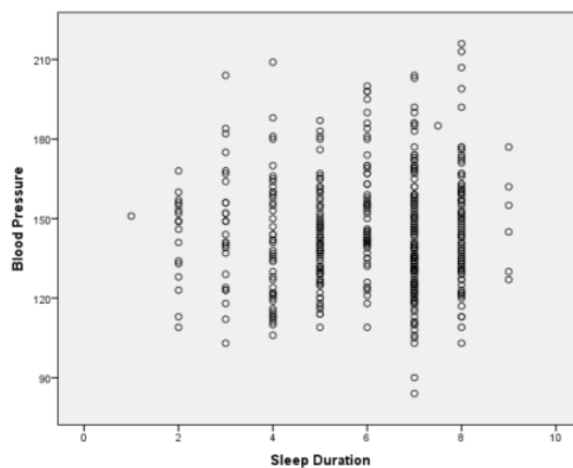
29 Figure 2: Scatter Plot of Systolic Blood Pressure and Sleep Duration
