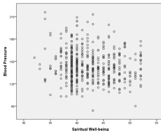
32 Figure 1: Scatter Plot of Systolic Blood Pressure and Spiritual Well-Being
