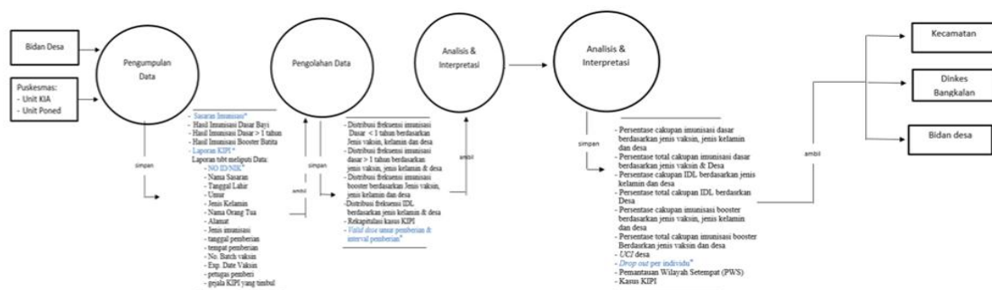
Gambar 2. DFD Level 0
