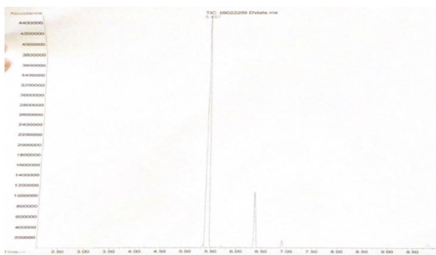
Figure 1. Chromatogram of clove leaf essential oil
