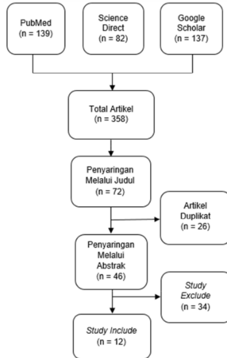
Gambar 1. Diagram PRISMA
