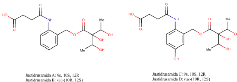
Figure 6. Alkaloid structure of Justicia gendarussa Burm. f.
