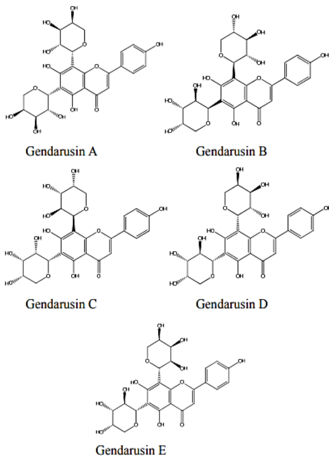
Figure 4. The structure of gendarusin compounds in Justicia gendarussa Burm. f.
