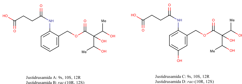
Figure 6. Alkaloid structure of Justicia gendarussa Burm. f.
