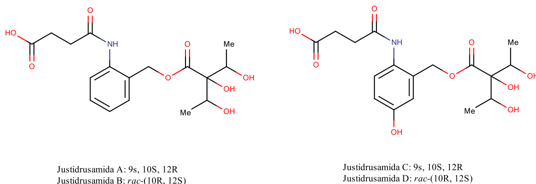
Figure 6. Alkaloid structure of Justicia gendarussa Burm. f.
