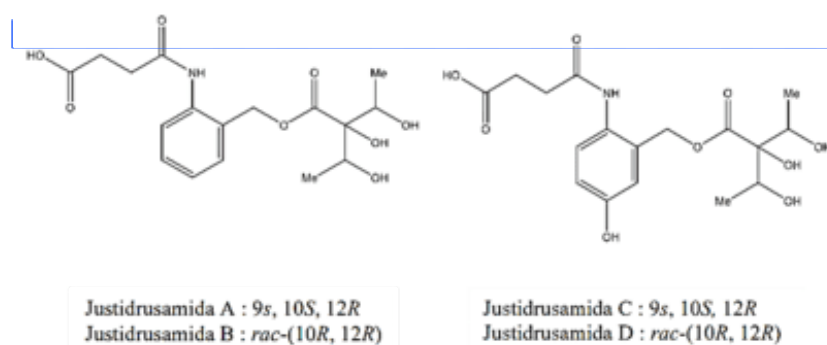
Figure 5. Alkaloid structure of Justicia gendarussa Burm. f.
