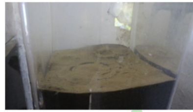
Figure 4. Schmutzdecke layer in slow sand filter.
