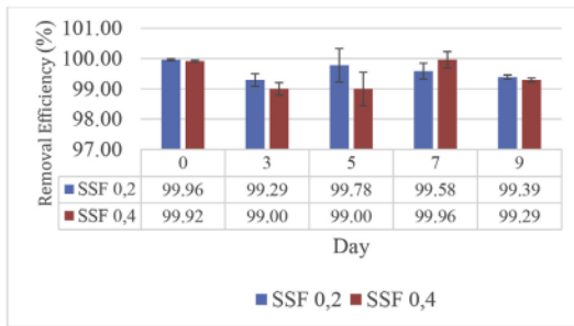
Figure 3. Coliform removal efficiency of slow sand filter.
