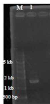
Figure 2. Amplicon of 18S rDNA using primer universal NS1 and NS8. M= Marker, I = T1P2
