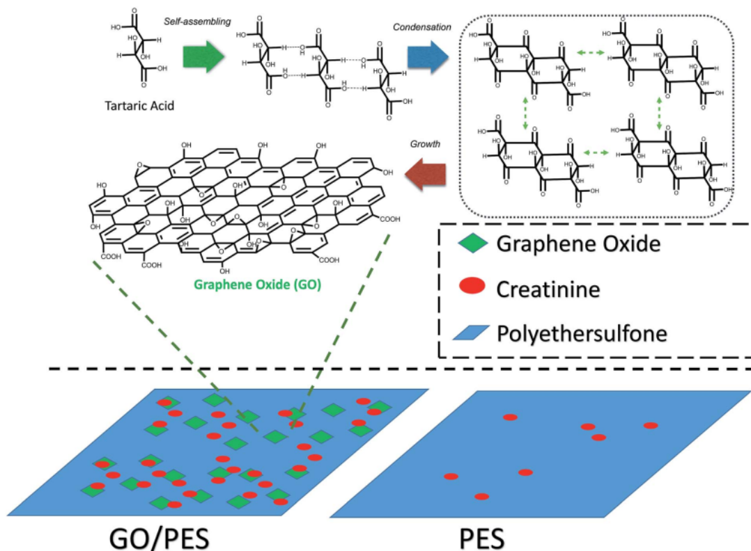
Scheme 1 Schematic mechanism of GO formation.
