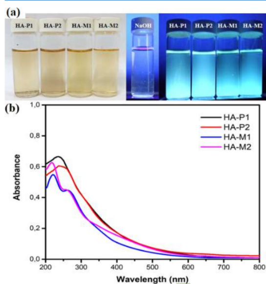
Figure 1. (a) Photograph of HA CDs taken under 320 nm UV light. (b) UV-vis spectra of furnace-assisted CDs, which are referred to as HA-P1 (black line) and HA-P2 (red line). UV-vis spectra of the microwave-assisted CDs, referred to as HA-M1 (blue line) and HA-M2 (purple line).
