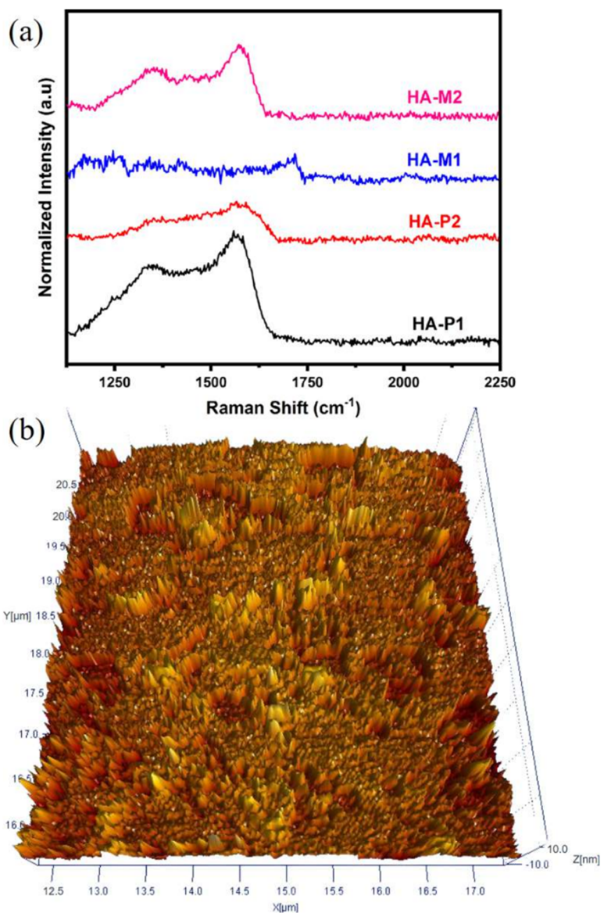
Figure 5. (a) Raman spectra of microwave-assisted CDs HA-M2 (purple line) and HA-M1 (blue line) and furnace-assisted CDs HA-P2 (red line) and HA-P1 (black line). (b) 3D topography of HA-P2.
