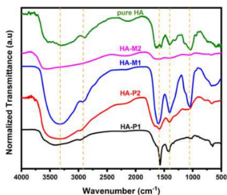
Figure 3. IR data of pure HA (green line), microwave-assisted CDs HA-M2 (purple line) and HA-M1 (blue line), and furnace-assisted CDs HA-P2 (red line) and HA-P1 (black line).
