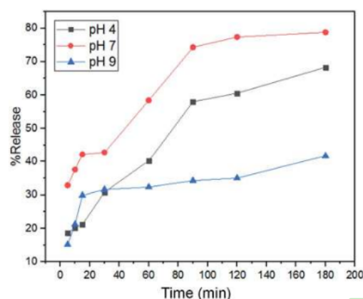
41 Fig. 8 The dissolution test of naproxen-loaded BCD under pH 4 (black line), 7 (red line), and 9 (blue line) buffer conditions ( t = 3 h, with \pm SD n = 3 ).
