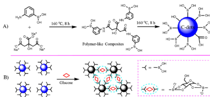
Figure 10. Schematic diagram of the synthesis process to fabricate boronic-acid-functionalized C-dots (A) and the interaction of CDs between boronic acid and cis -diol groups for glucose sensing (B). Reproduced with permission from ref 17. Copyright 2018 Elsevier B.V.
