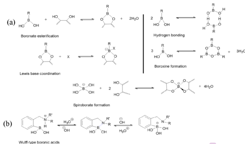
Scheme 3. Main Boronic Acid Interactions Concerning the Self-Assembly (a) and Intramolecular Interaction between Boronic Acid and a Nitrogen Atom (b) 49
