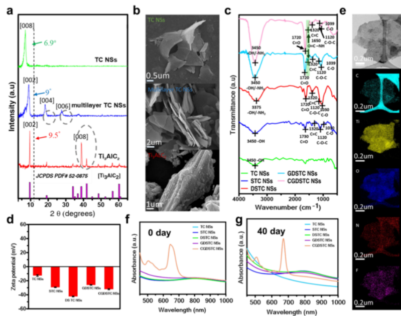
Figure 2. (a) XRD spectra and (b) SEM of Ti_3AlC_2 , multilayer TC NSs, and TC NSs. (c) FT-IR spectra and (d) zeta potential measurements of TC NSs, STC NSs, DSTC NSs, GDSTC NSs, and CGDSTC NSs. (e) HRTEM and elemental mapping images (C, Ti, O, N, and F) of CGDSTC NSs. UV-Vis spectra of TC NSs, STC NSs, DSTC NSs, GDSTC NSs, and CGDSTC NSs (f) for 0 day storage and (g) after 40 days storage (stored at room temperature).
