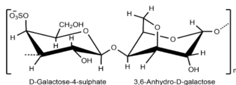
Figure 3: Structure of \kappa -carrageenan
