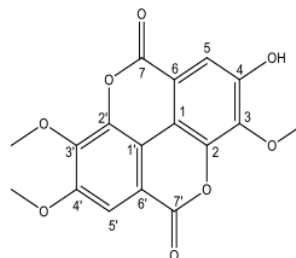
Figure 1: Structure of 3,4,3'-tri- O -methyl ellagic acid
