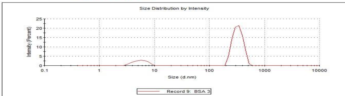
Gambar 9. Spektra BSA
