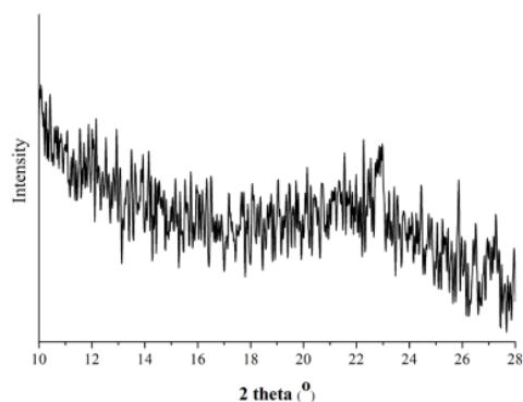
Fig. 4. XRD pattern of FC300.
