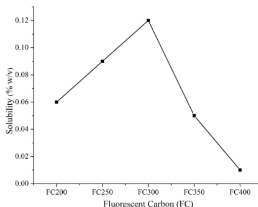
Fig. 1. Solubility of fluorescent carbons (FC).
