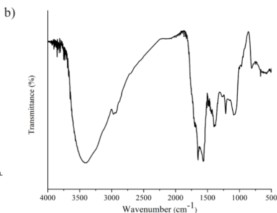
Fig. 5. FTIR Spectrum of FC300.
