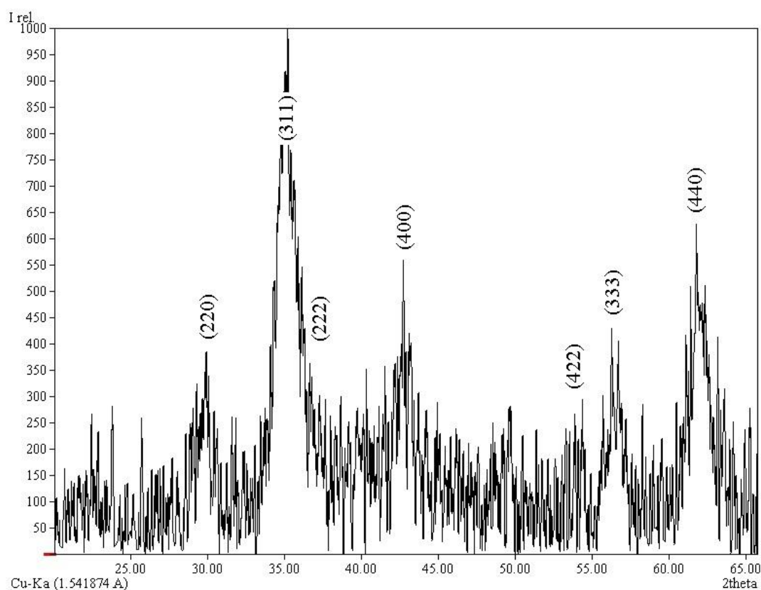
Figure 1. XRD pattern of prepared MF NPs.
