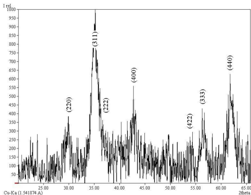
Figure 1. XRD pattern of prepared MF NPs.
