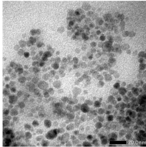
Figure 2. TEM micrograph of MF NPs.
