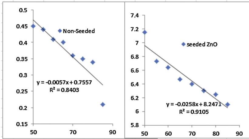
Fig. 6. Sensing results for the proposed relative humidity sensor using a tapered POF coated with ZnO nanostructure.
