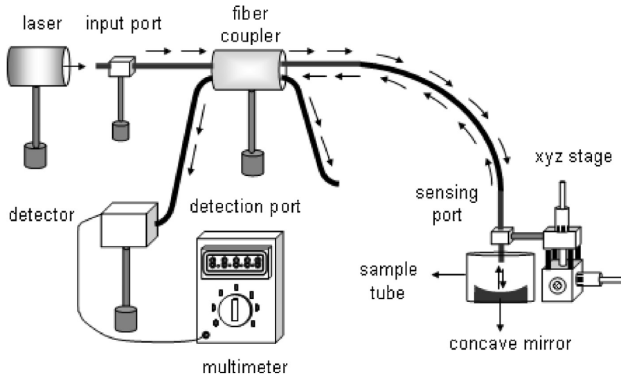
Fig. 2. Experimental setup for magnesium ion concentration sensor.
