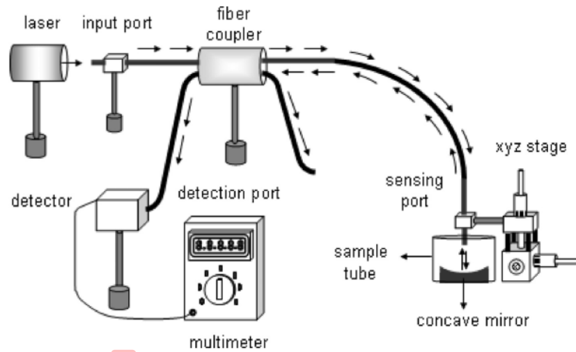
Fig. 2. Experimental setup for magnesium ion concentration sensor.
