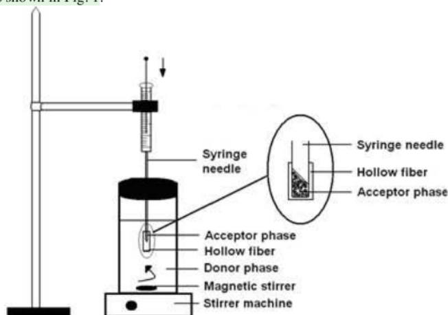
Fig.1. Device of HF-LPME
