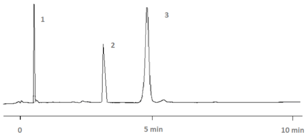
Fig.2. Chromatogram of 1) methanol; 2) NDEA; and 3) NDPA Conditions: Concentration of NDEA and NDPA mixture 20 \text{mg L}^{-1} ; carrier gas: nitrogen; column flow: 40 \text{mL}\cdot\text{min}^{-1}
