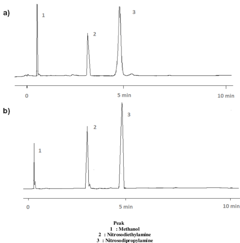
Fig.7: Chromatograms of: a) original real sample and b) spiked samples
