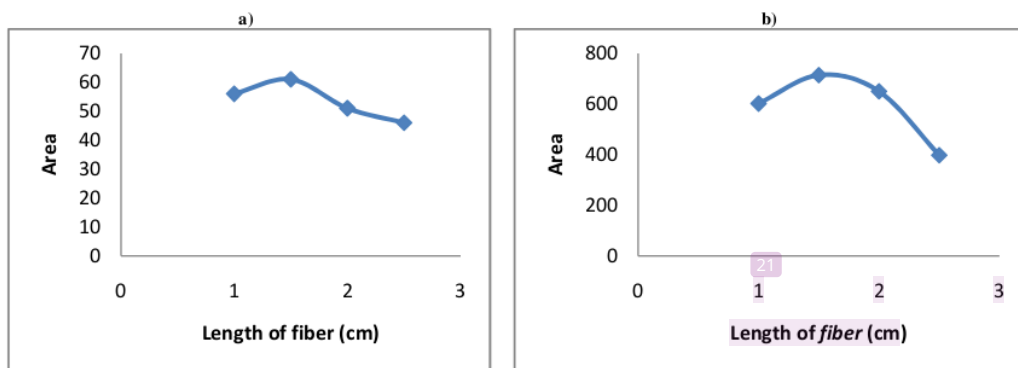
Fig.5. Length of fiber effect for the a) NDEA and b) NDPA used in this study
