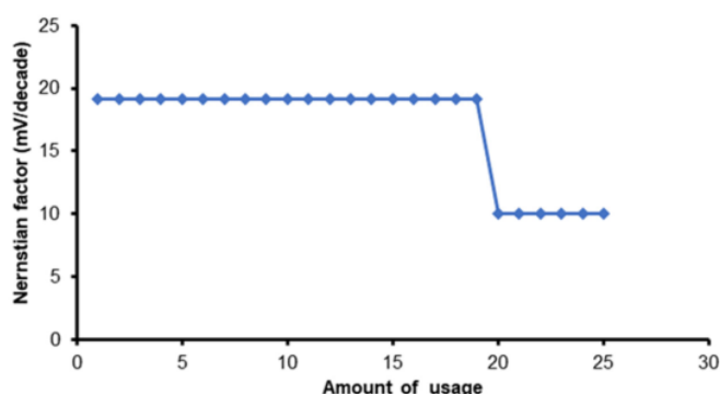
Fig 6. Lifetime electrode graph
