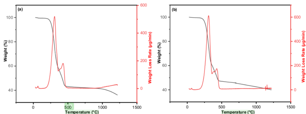
Fig 4. TGA/DTG of (a) MIP and (b) NIP
