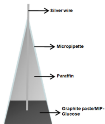
Fig 1. Electrode construction
