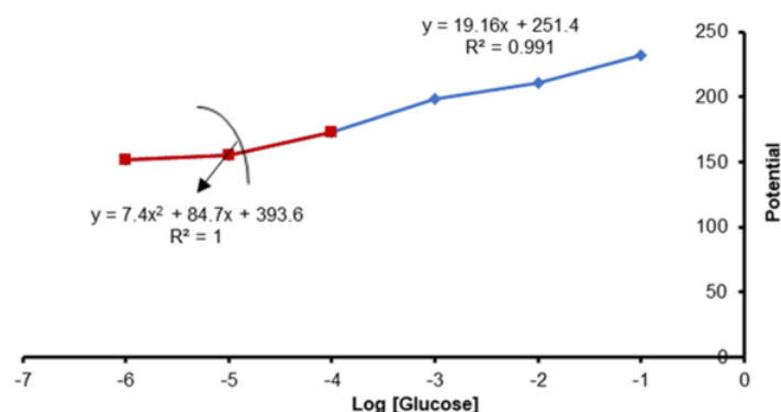
Fig 5. Detection limit measurement curve
