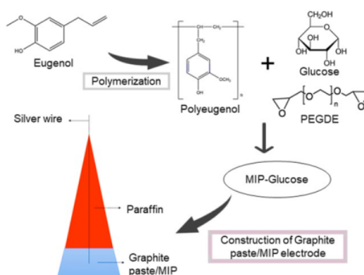
Fig 1. Graphite paste/MIP electrode synthesis
