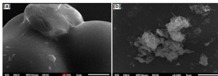
Fig 4. SEM results of (a) NIP (b) IP
