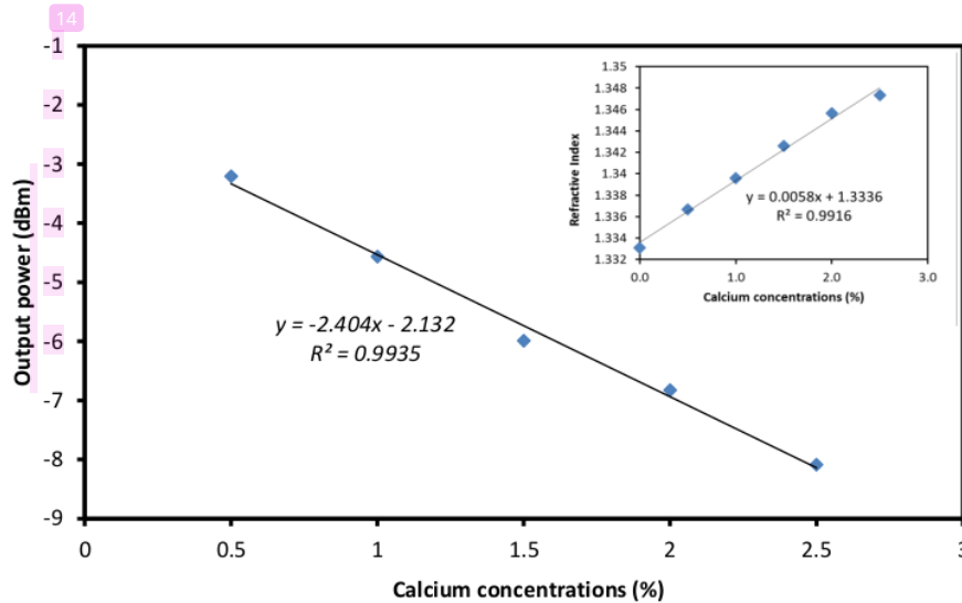
Fig. 6. The output power of the ASE against calcium concentrations. Inset shows refractive index of the solution at different calcium concentrations
