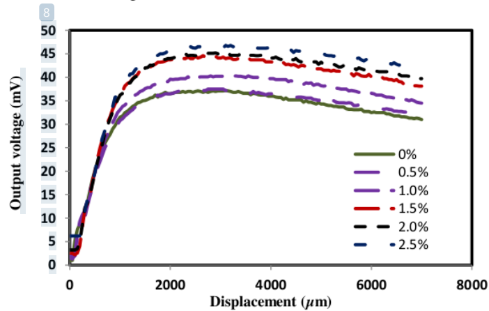
Fig. 4. Output voltage of the sensor (mV) as function of displacement ( \mu\text{m} ) for various calcium concentration
