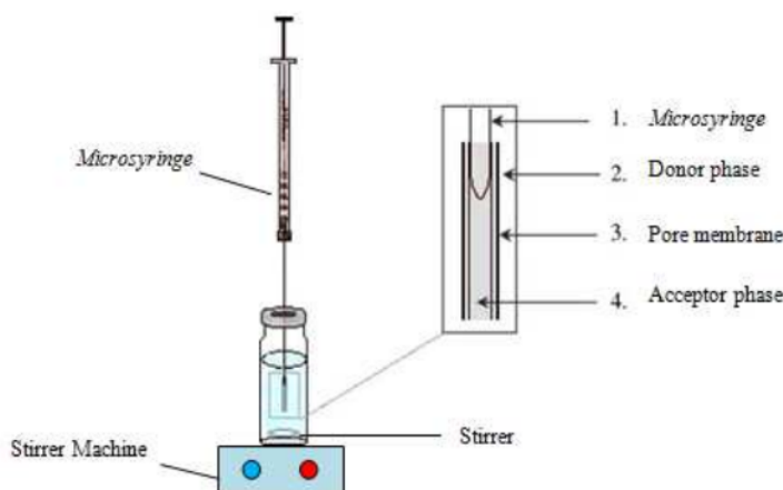
Picture 1. Set-up HF-LPME
