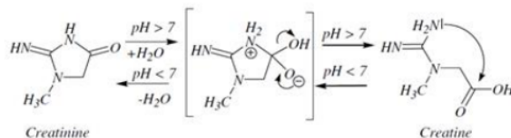
Figure 2. Prediction of of creatine reduction reaction [8]
