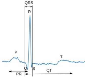
Fig. 1: Electrocardiogram signal
