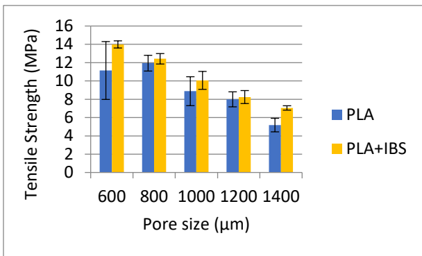
Fig. 5. The tensile strength test result
