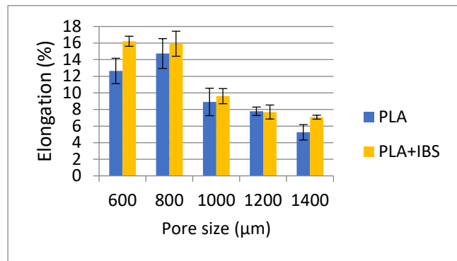
Fig. 6. The elongation test result
