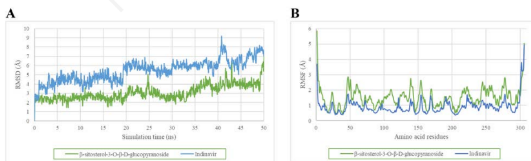
Figure 3. Root Mean Square Deviation (RMSD) plot exhibits that \beta -sitosterol-3-O- \beta -D-glucopyranoside has a lower RMSD value, meaning the complex ligand-receptor has more stable than Indinavir (A). However, \beta -sitosterol-3-O- \beta -D-glucopyranoside has a higher Root Mean Square Fluctuation (RMSF) that reflects the amino acids are fluctuative quite value than Indinavir but is still on the acceptable threshold ( <3 Å) (B). It can be known that \beta -sitosterol-3-O- \beta -D-glucopyranoside is stably bound to the 3Clpro SARS-CoV-2 receptor for 50 ns simulation times.
