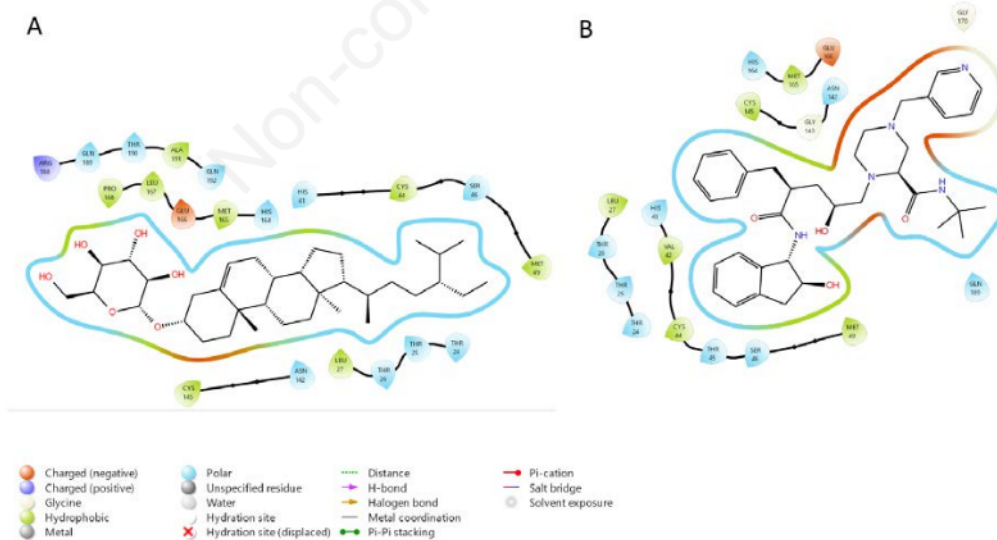
Figure 2. Molecular interactions of \beta -sitosterol-3-O- \beta -D-glucopyranoside (A) and Indinavir (B) against binding sites of 3Clpro SARS-CoV-2. Both compounds interacted with catalytic sites suggesting being active as 3Clpro inhibitors.
