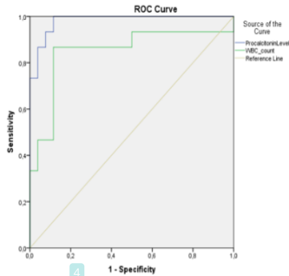
4 Figure 1. The Receiver Operating Characteristic (ROC) Curve Analysis of Procalcitonin (PCT) and White Blood Cell (WBC) Count
