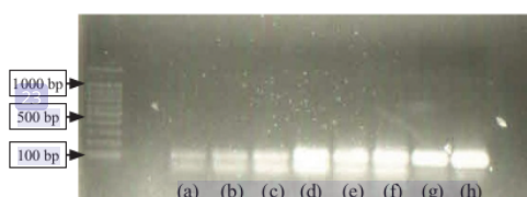
Figure 2. Electrophoresis on 1.5% agarose of RT-PCR after treatment, molecular weight marker (100 bp), (a) treatment with 50 \mu\text{g/ml} compound, (b) 25 \mu\text{g/ml} , (c) 12.5 \mu\text{g/ml} , (d) 6.25 \mu\text{g/ml} , (e) 3.13 \mu\text{g/ml} , (f) 1.57 \mu\text{g/ml} , (g) 0.78 \mu\text{g/ml} , and (h) 0.39 \mu\text{g/ml}
