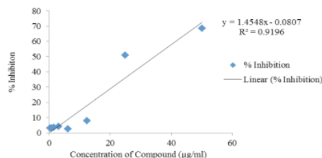
Figure 1. Inhibition of DENV-2, at variation concentrations of Zinc(II)-2,4,5-triphenyl-1 H -imidazole complex compound
