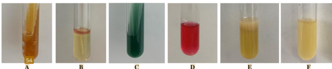
Figure 2. Identification results of Escherichia coli in the TSIA, IMViC, and Urease Biochemical tests. A. TSIA, B. SIM, C. Citrate, D. MR, E. VP, F. Urease
