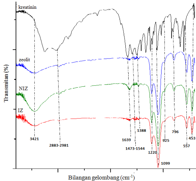
Gambar 5.4 Spektra FTIR kreatinin, zeolit, non-imprinted zeolit, dan imprinted zeolit
