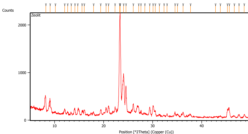
Figure 1 Diffractogram of TS-1 zeolite
