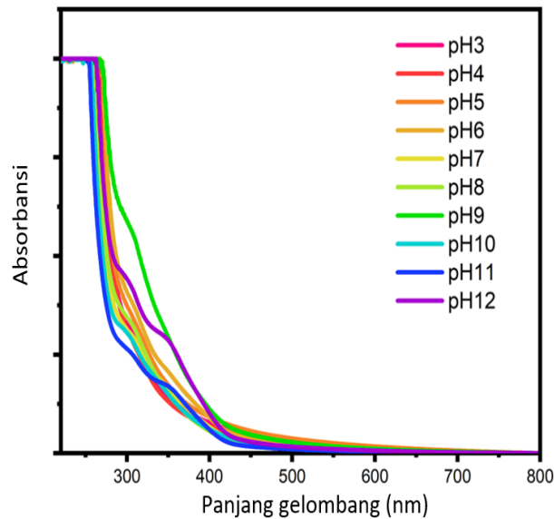
Gambar 11. Spektra UV karbon dot B-CDs2 variasi pH 3-12
